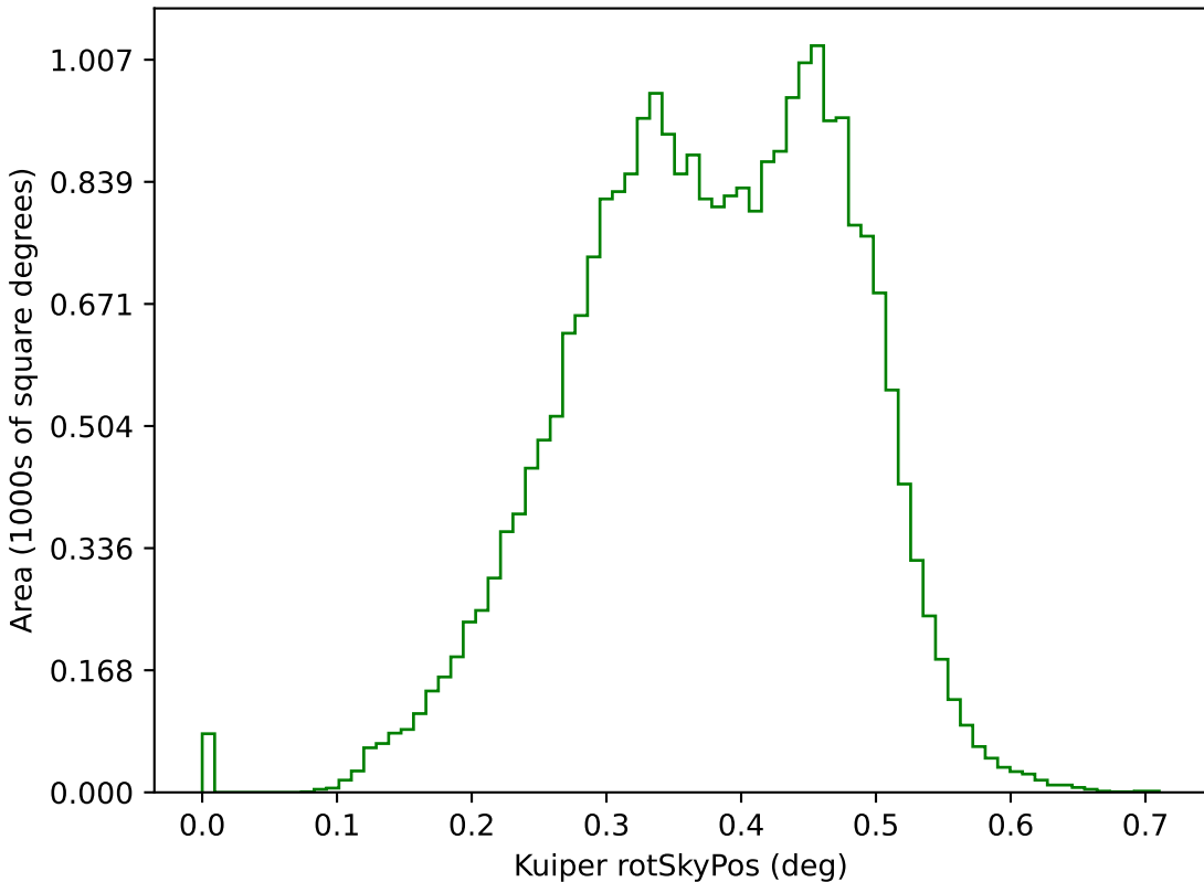
too_elab_r32_d2_gz_v3.4_10yrs g: Kuiper rotSkyPos
