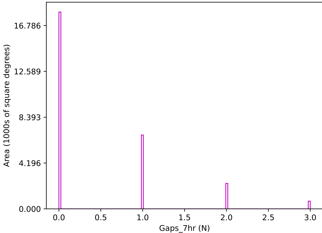
too_elab_r32_d2_gz_v3.4_10yrs z band: Gaps_7hr
