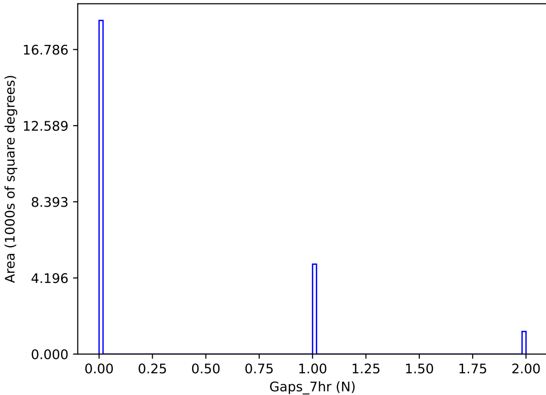
too_elab_r32_d2_gz_v3.4_10yrs y band: Gaps_7hr
