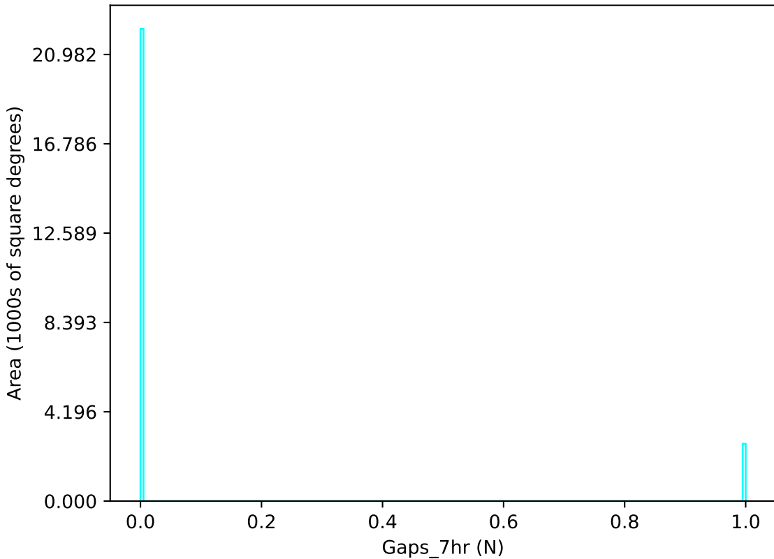
too_elab_r32_d2_gz_v3.4_10yrs u band: Gaps_7hr
