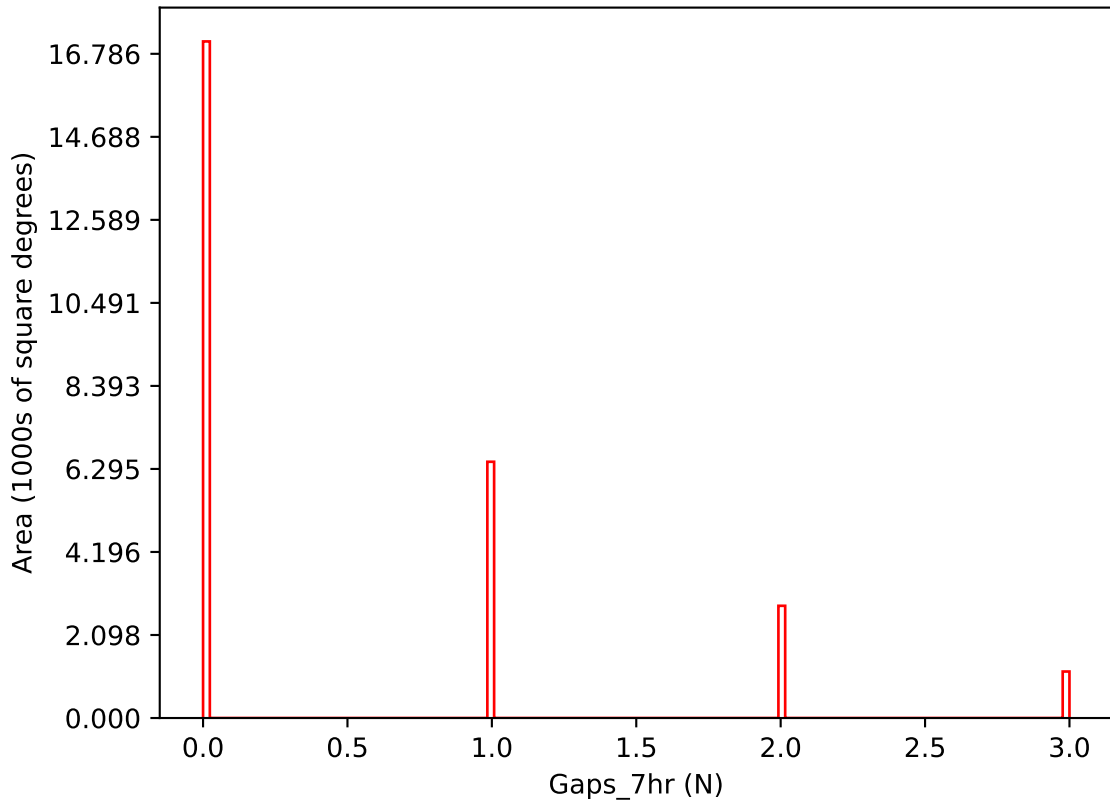
too_elab_r32_d2_gz_v3.4_10yrs i band: Gaps_7hr
