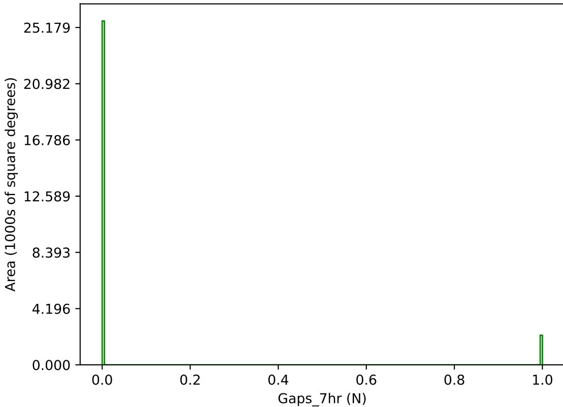
too_elab_r32_d2_gz_v3.4_10yrs g band: Gaps_7hr
