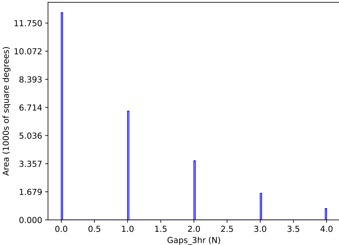
too_elab_r32_d2_gz_v3.4_10yrs y band: Gaps_3hr
