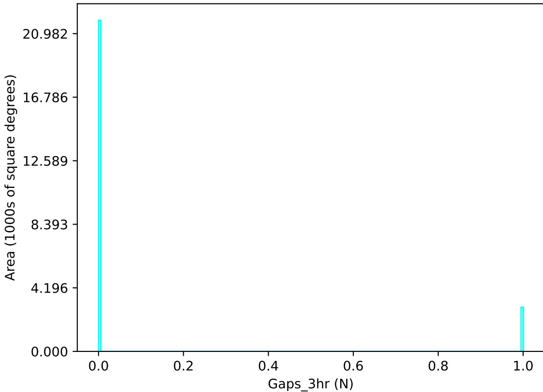
too_elab_r32_d2_gz_v3.4_10yrs u band: Gaps_3hr
