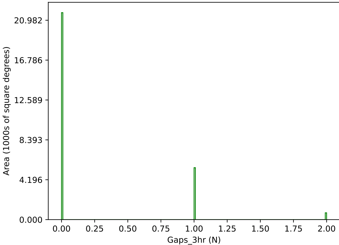
too_elab_r32_d2_gz_v3.4_10yrs g band: Gaps_3hr
