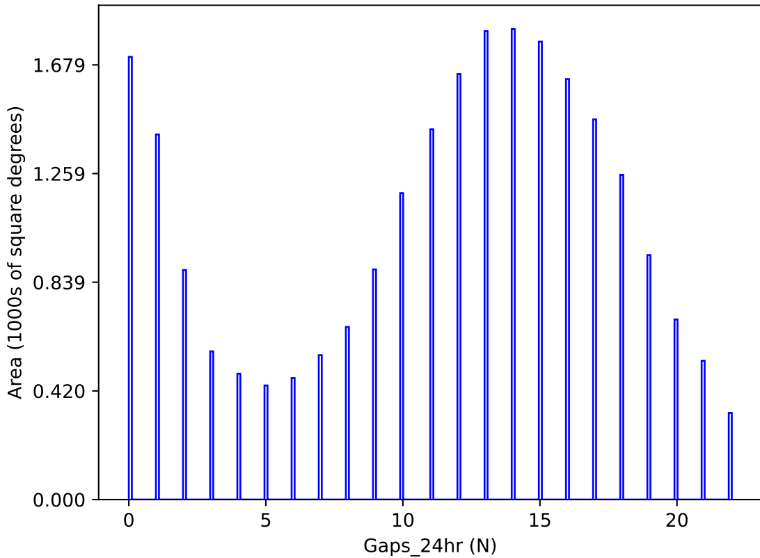
too_elab_r32_d2_gz_v3.4_10yrs y band: Gaps_24hr
