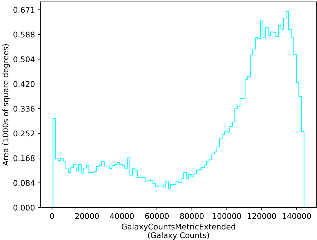
too_elab_r32_d2_gz_v3.4_10yrs u: GalaxyCountsMetricExtended
