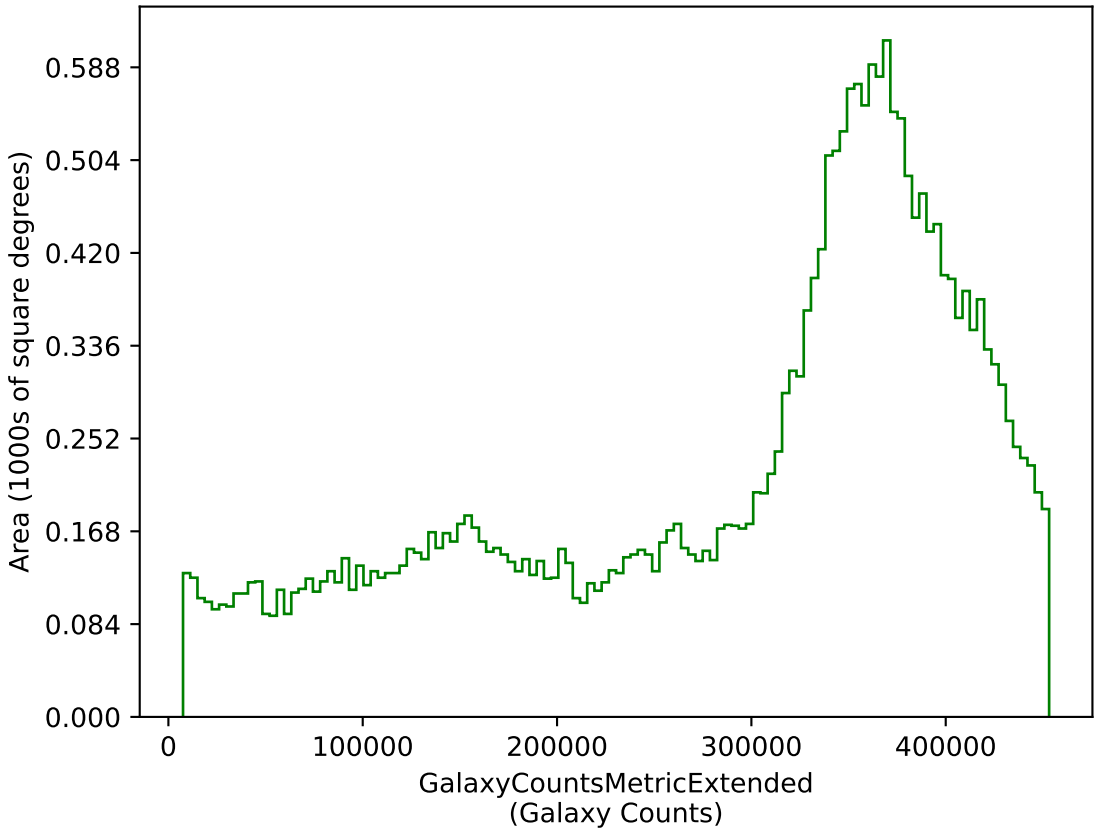
too_elab_r32_d2_gz_v3.4_10yrs g: GalaxyCountsMetricExtended
