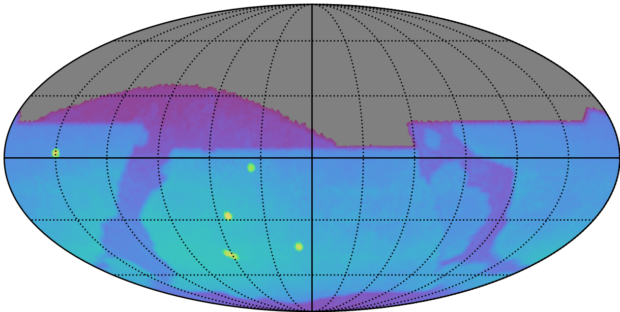
too_elab_r32_d2_gz_v3.4_10yrs : Brown Dwarf, L7
