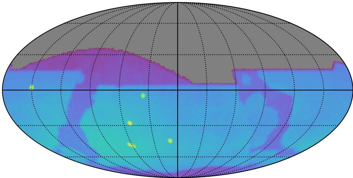
too_elab_r32_d2_gz_v3.4_10yrs : Brown Dwarf, L4
