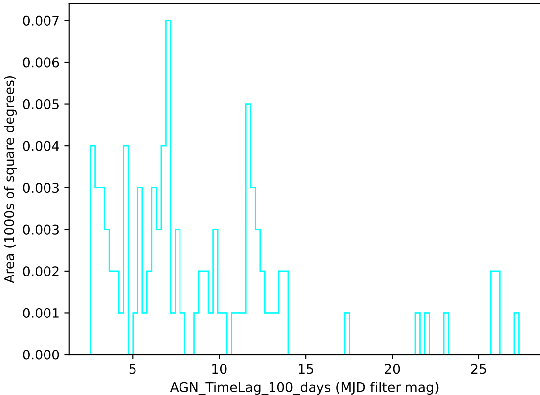
too_elab_r32_d2_gz_v3.4_10yrs u band: AGN_TimeLag_100_days
