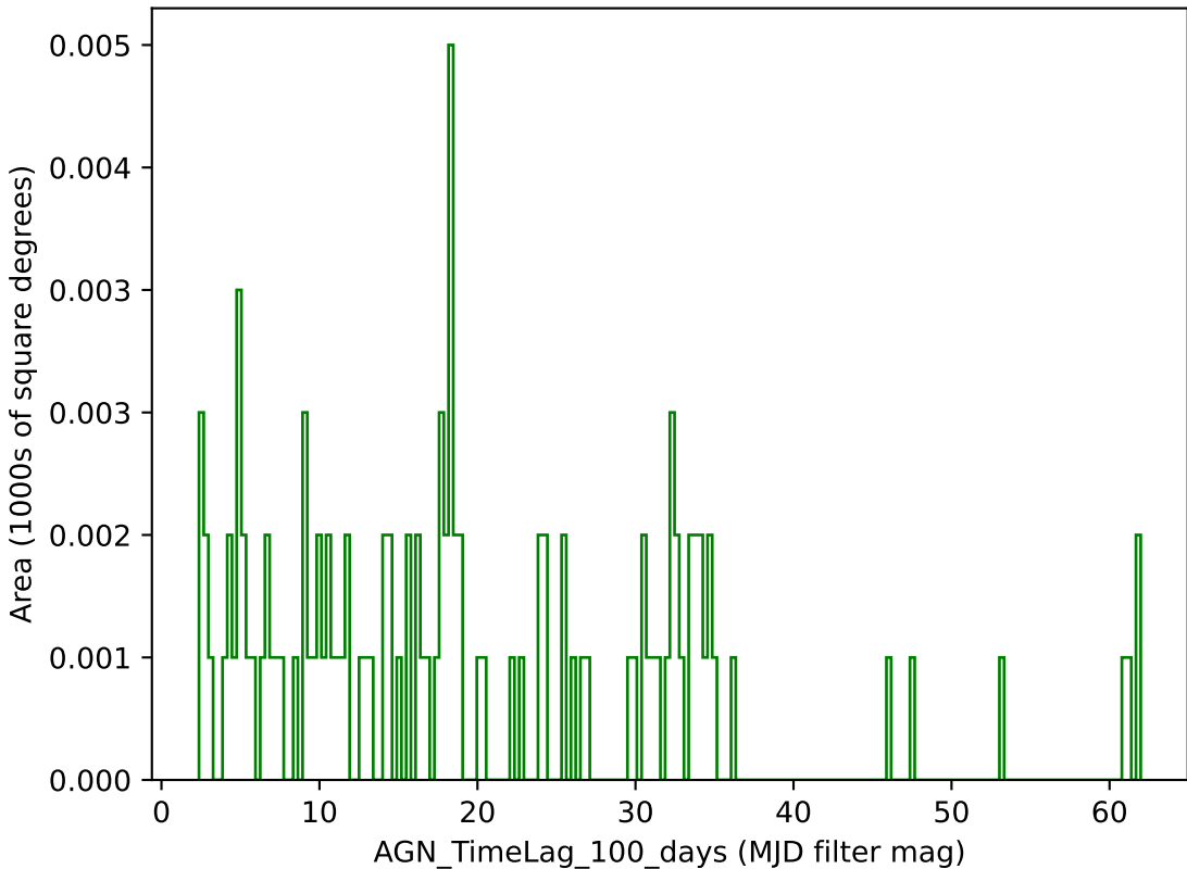
too_elab_r32_d2_gz_v3.4_10yrs g band: AGN_TimeLag_100_days
