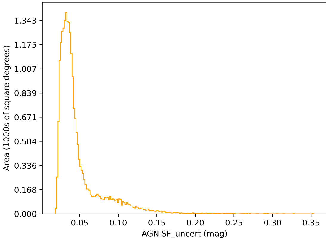
too_elab_r32_d2_gz_v3.4_10yrs r band: AGN SF_uncert
