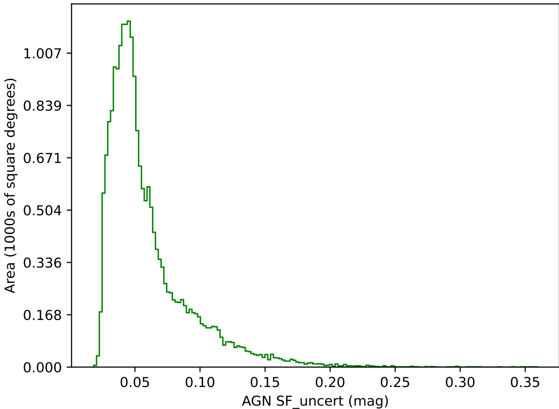
too_elab_r32_d2_gz_v3.4_10yrs g band: AGN SF_uncert
