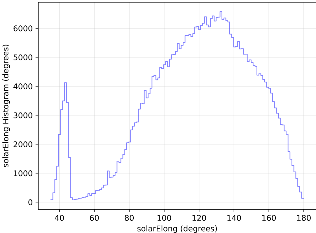
too_elab_r32_d2_gz_v3.4_10yrs WFD z band: solarElong Histogram
