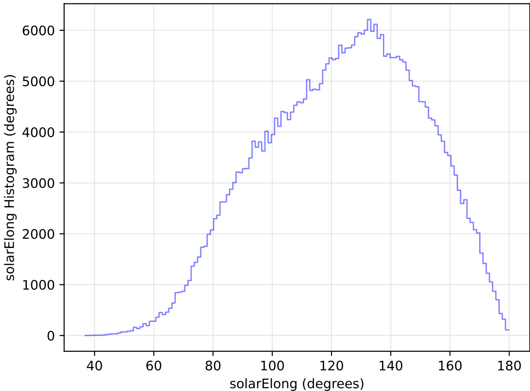
too_elab_r32_d2_gz_v3.4_10yrs WFD y band: solarElong Histogram
