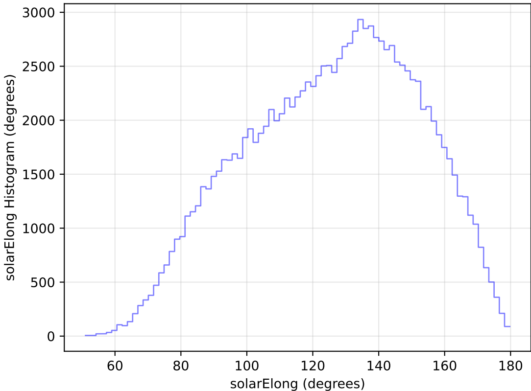
too_elab_r32_d2_gz_v3.4_10yrs WFD u band: solarElong Histogram
