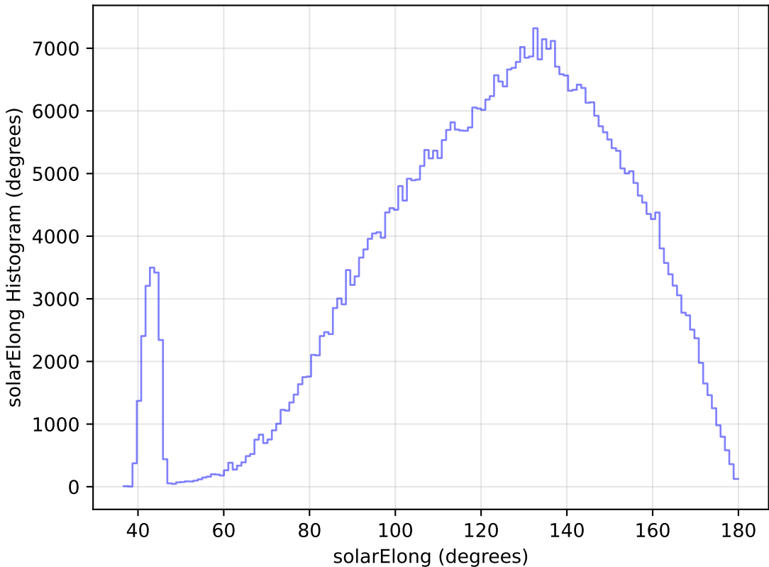
too_elab_r32_d2_gz_v3.4_10yrs WFD r band: solarElong Histogram
