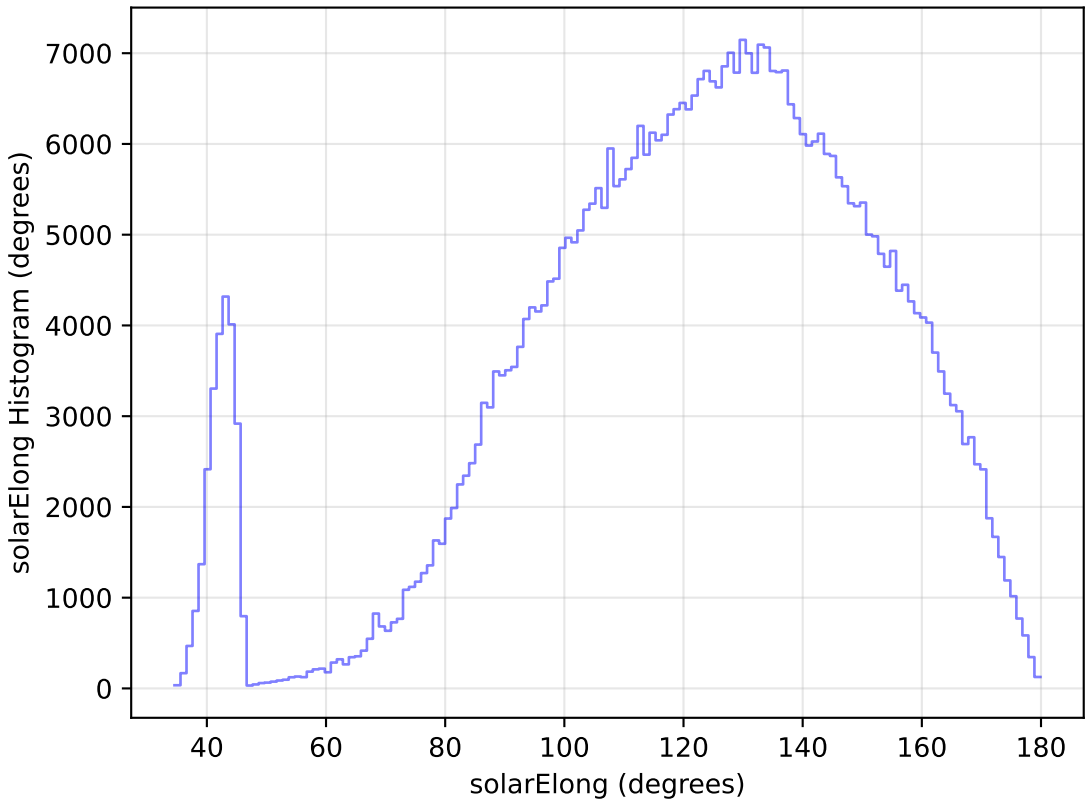
too_elab_r32_d2_gz_v3.4_10yrs WFD i band: solarElong Histogram
