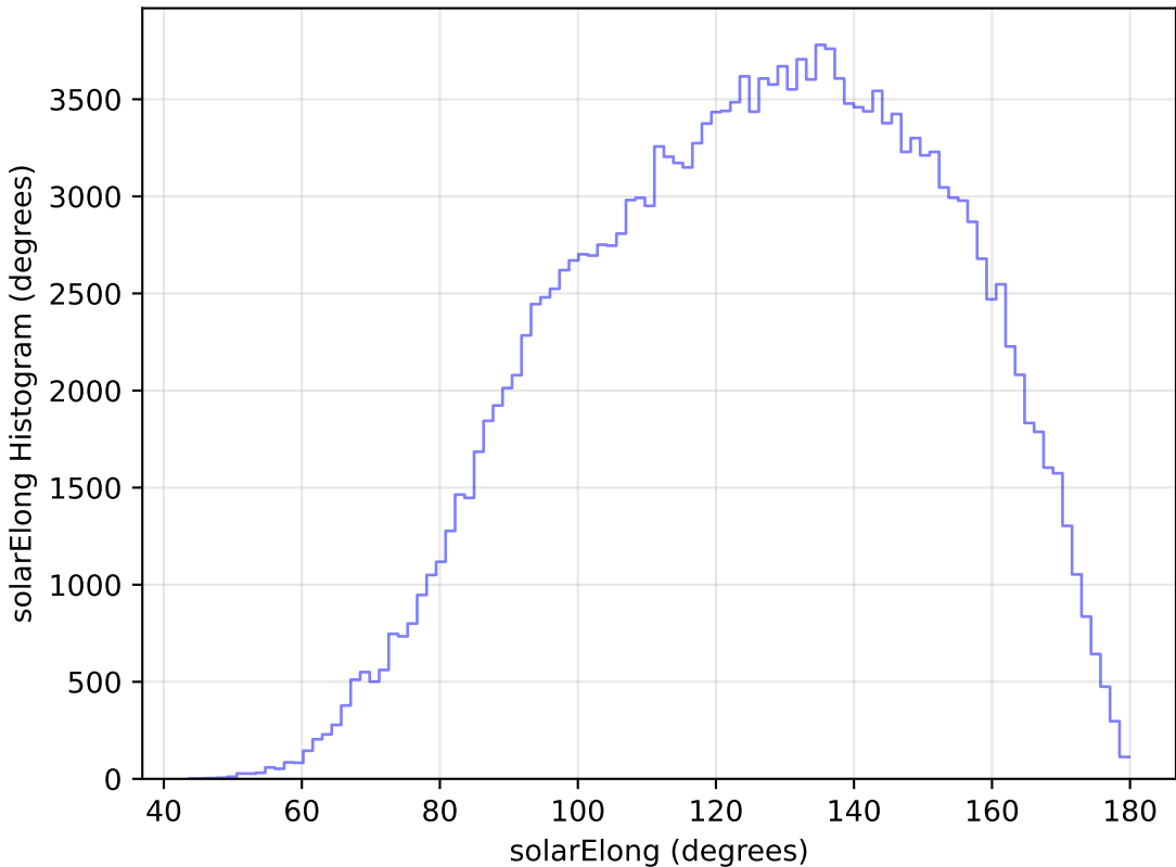
too_elab_r32_d2_gz_v3.4_10yrs WFD g band: solarElong Histogram
