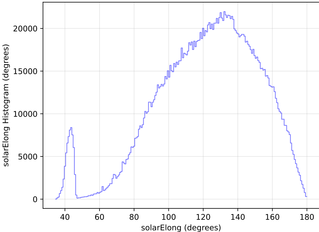
too_elab_r32_d2_gz_v3.4_10yrs WFD all bands: solarElong Histogram
