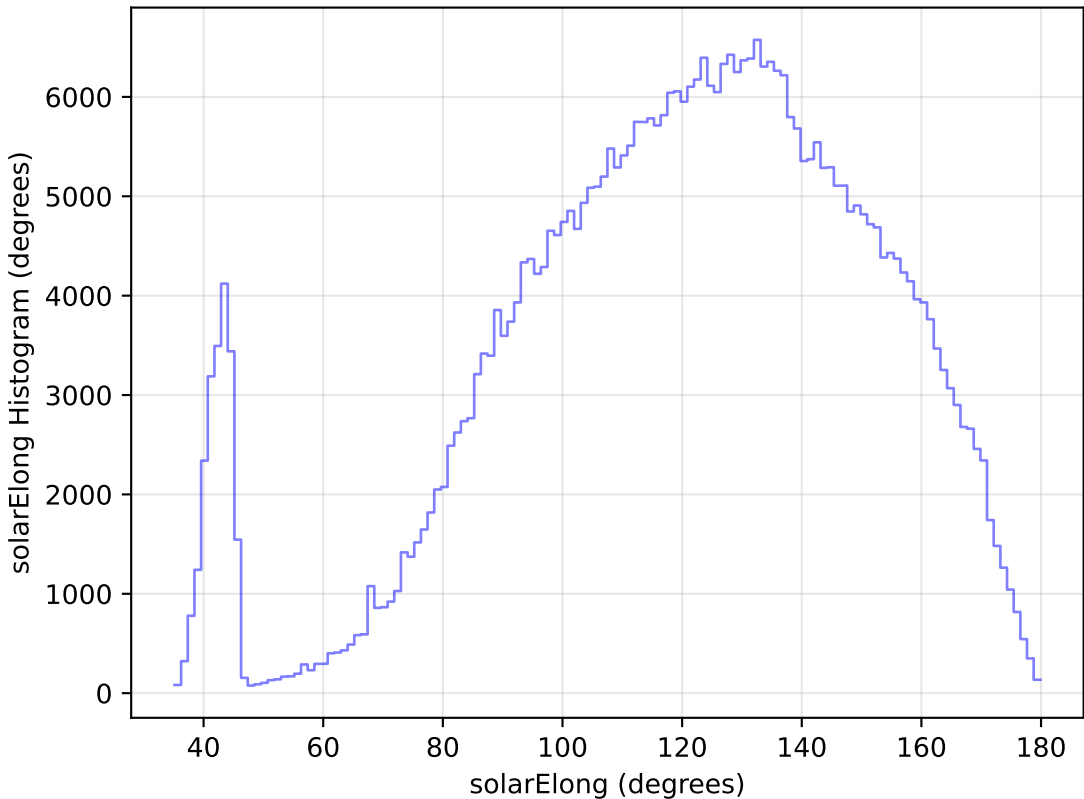
too_elab_r32_d2_gz_v3.4_10yrs All sky z band: solarElong Histogram
