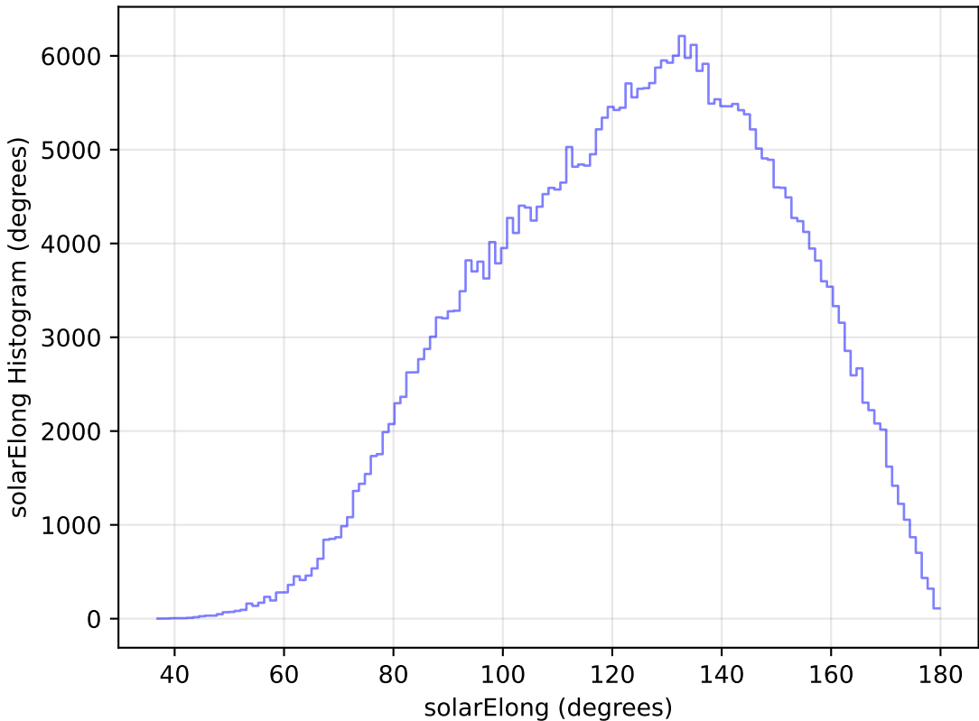
too_elab_r32_d2_gz_v3.4_10yrs All sky y band: solarElong Histogram
