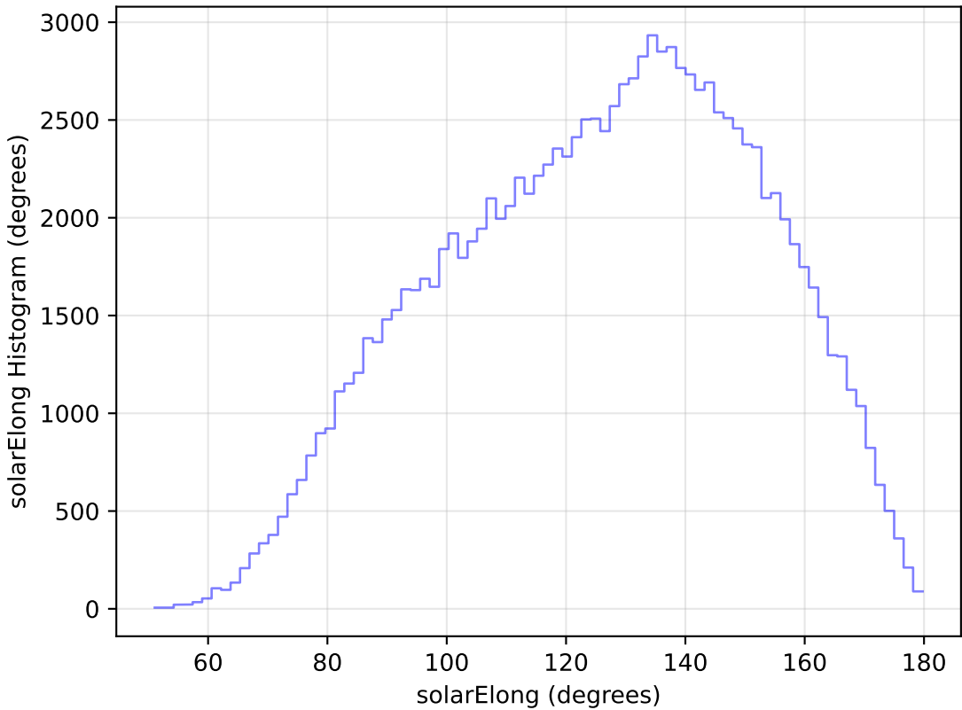
too_elab_r32_d2_gz_v3.4_10yrs All sky u band: solarElong Histogram
