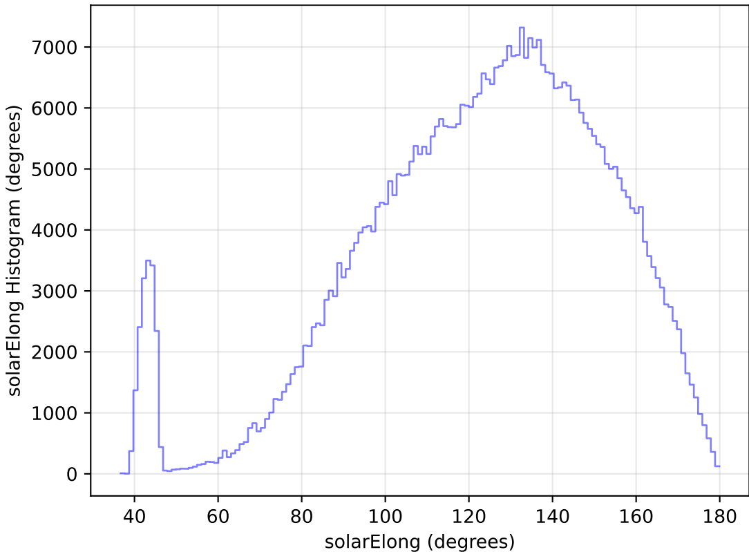
too_elab_r32_d2_gz_v3.4_10yrs All sky r band: solarElong Histogram
