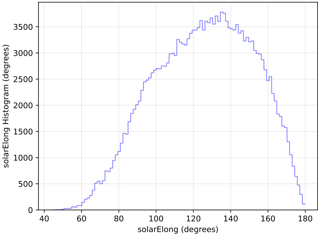
too_elab_r32_d2_gz_v3.4_10yrs All sky g band: solarElong Histogram
