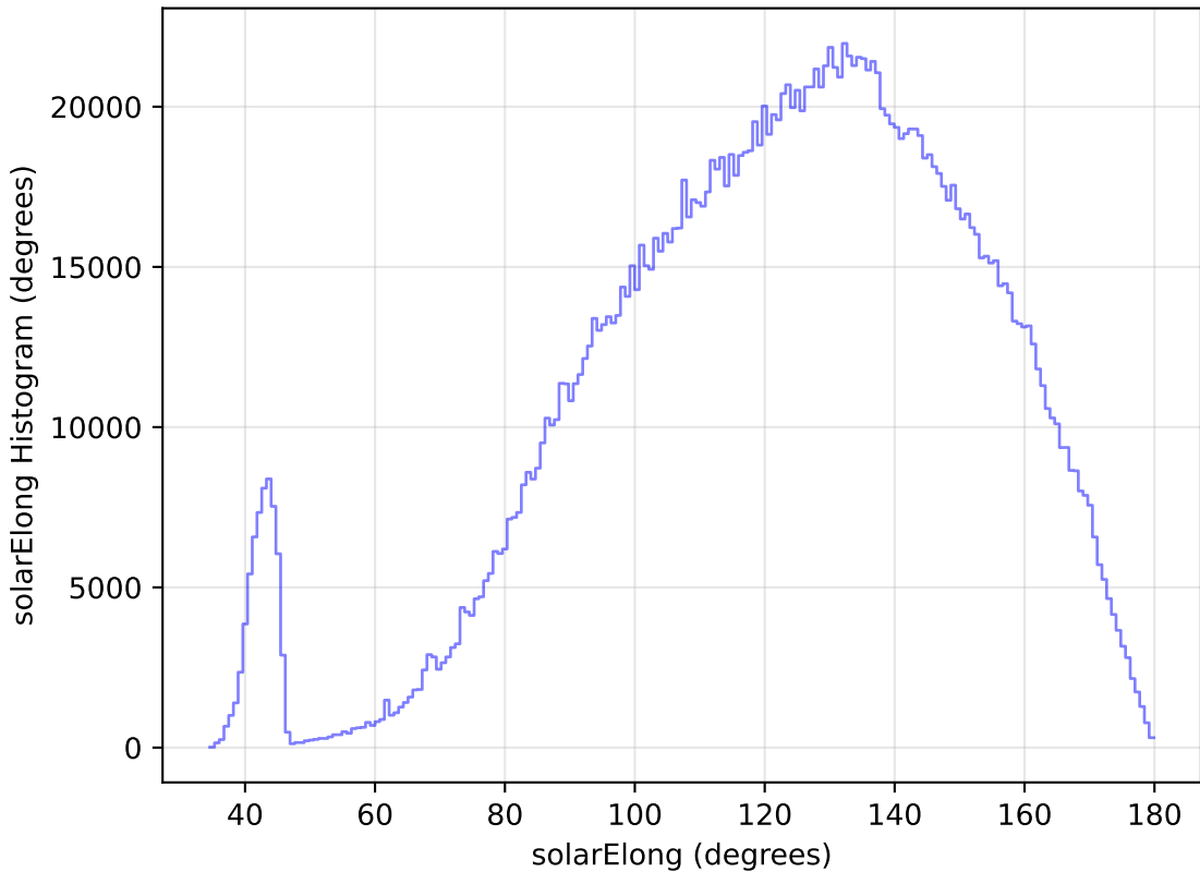
too_elab_r32_d2_gz_v3.4_10yrs All sky all bands: solarElong Histogram
