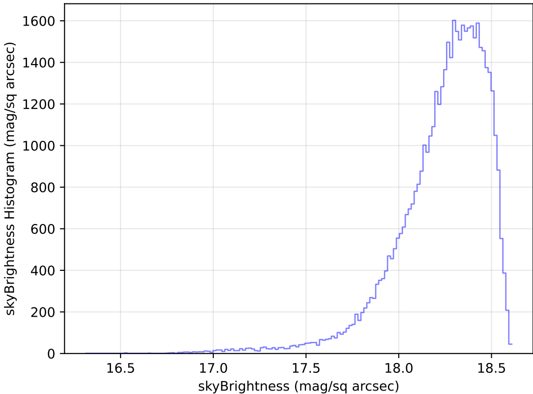
too_elab_r32_d2_gz_v3.4_10yrs Yr 1 y band: skyBrightness Histogram
