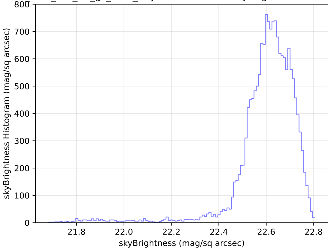
too_elab_r32_d2_gz_v3.4_10yrs Yr 1 u band: skyBrightness Histogram
