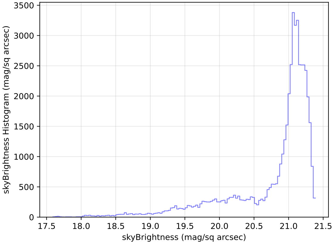
too_elab_r32_d2_gz_v3.4_10yrs Yr 1 r band: skyBrightness Histogram
