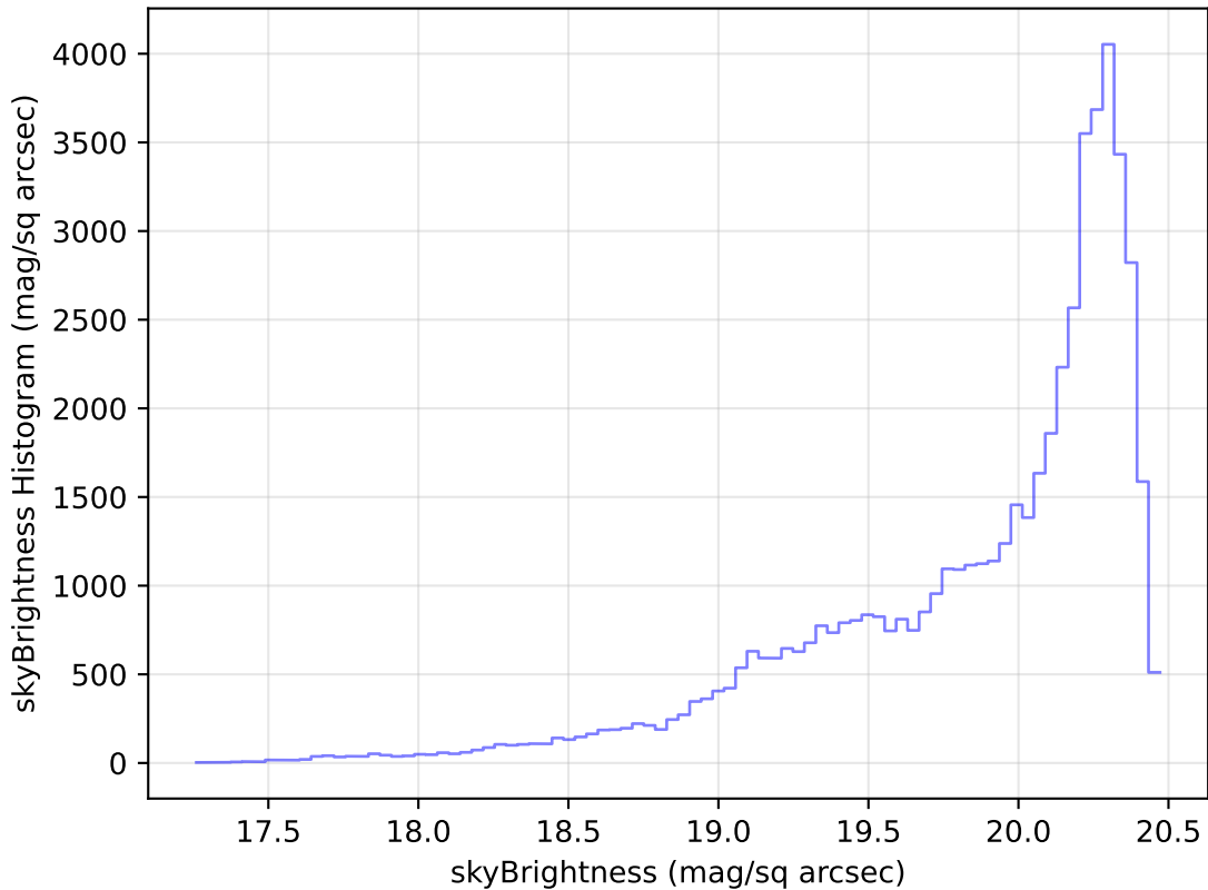
too_elab_r32_d2_gz_v3.4_10yrs Yr 1 i band: skyBrightness Histogram
