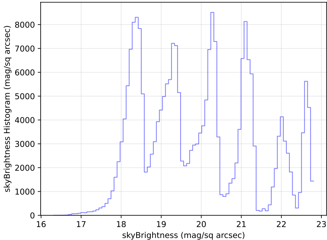
too_elab_r32_d2_gz_v3.4_10yrs Yr 1 all bands: skyBrightness Histogram
