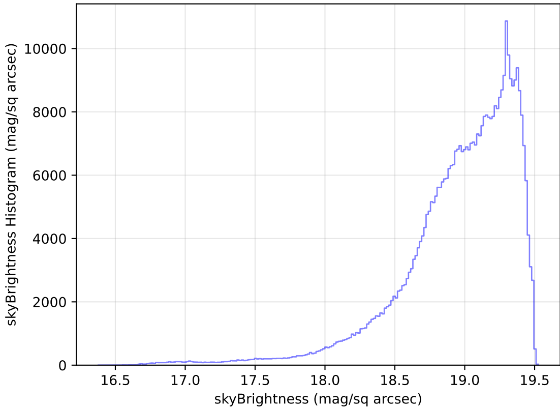
too_elab_r32_d2_gz_v3.4_10yrs WFD z band: skyBrightness Histogram
