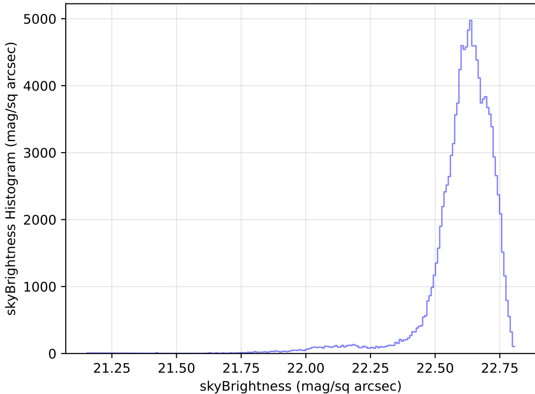
too_elab_r32_d2_gz_v3.4_10yrs WFD u band: skyBrightness Histogram
