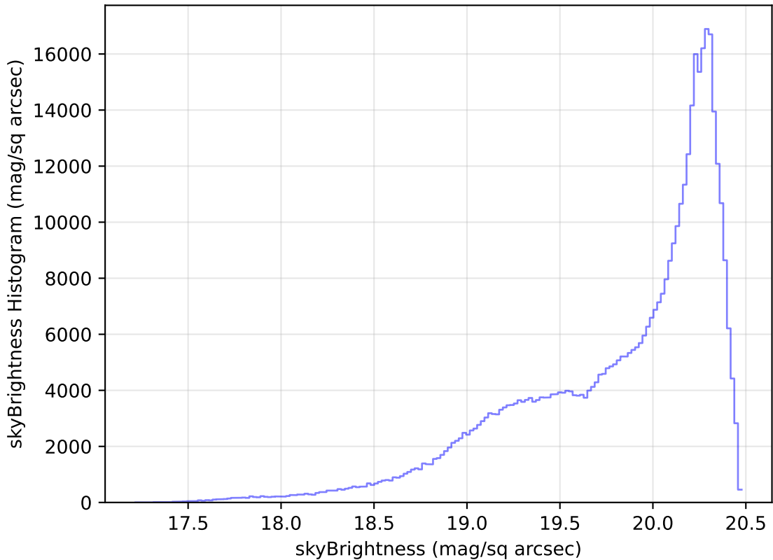
too_elab_r32_d2_gz_v3.4_10yrs WFD i band: skyBrightness Histogram
