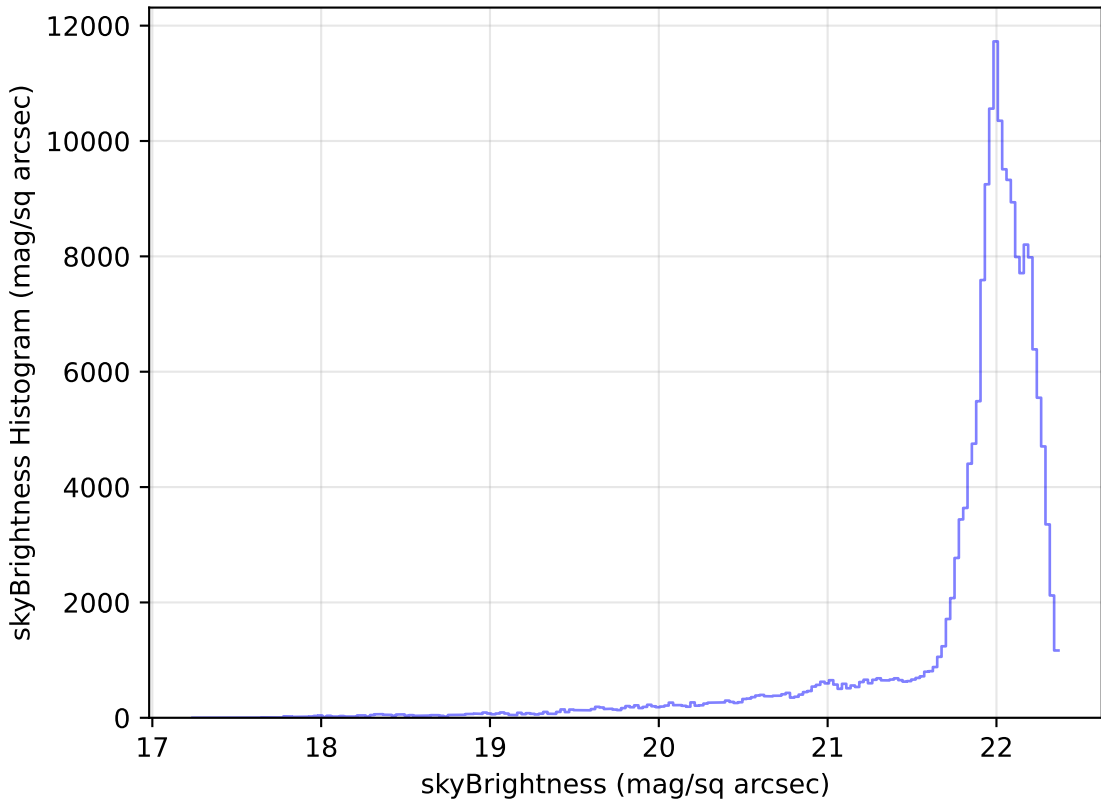
too_elab_r32_d2_gz_v3.4_10yrs WFD g band: skyBrightness Histogram
