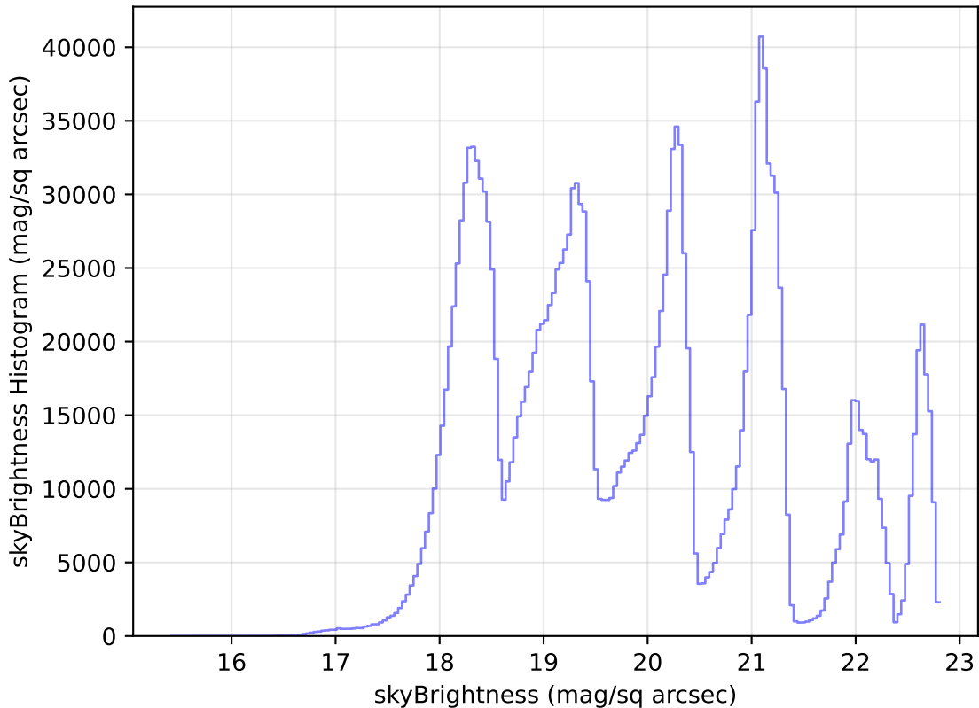
too_elab_r32_d2_gz_v3.4_10yrs WFD all bands: skyBrightness Histogram
