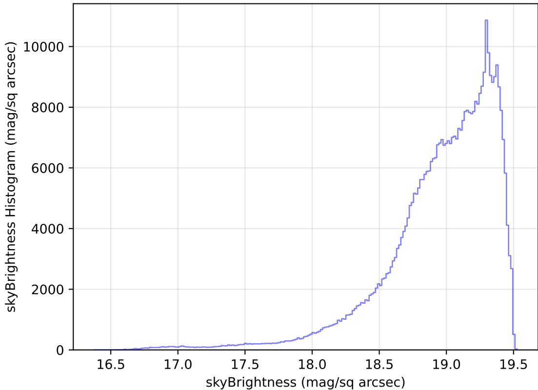
too_elab_r32_d2_gz_v3.4_10yrs All sky z band: skyBrightness Histogram
