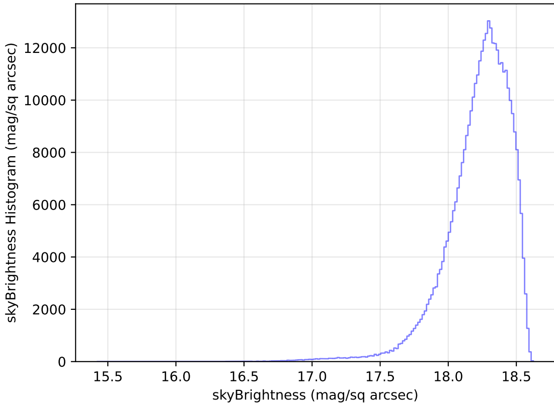
too_elab_r32_d2_gz_v3.4_10yrs All sky y band: skyBrightness Histogram
