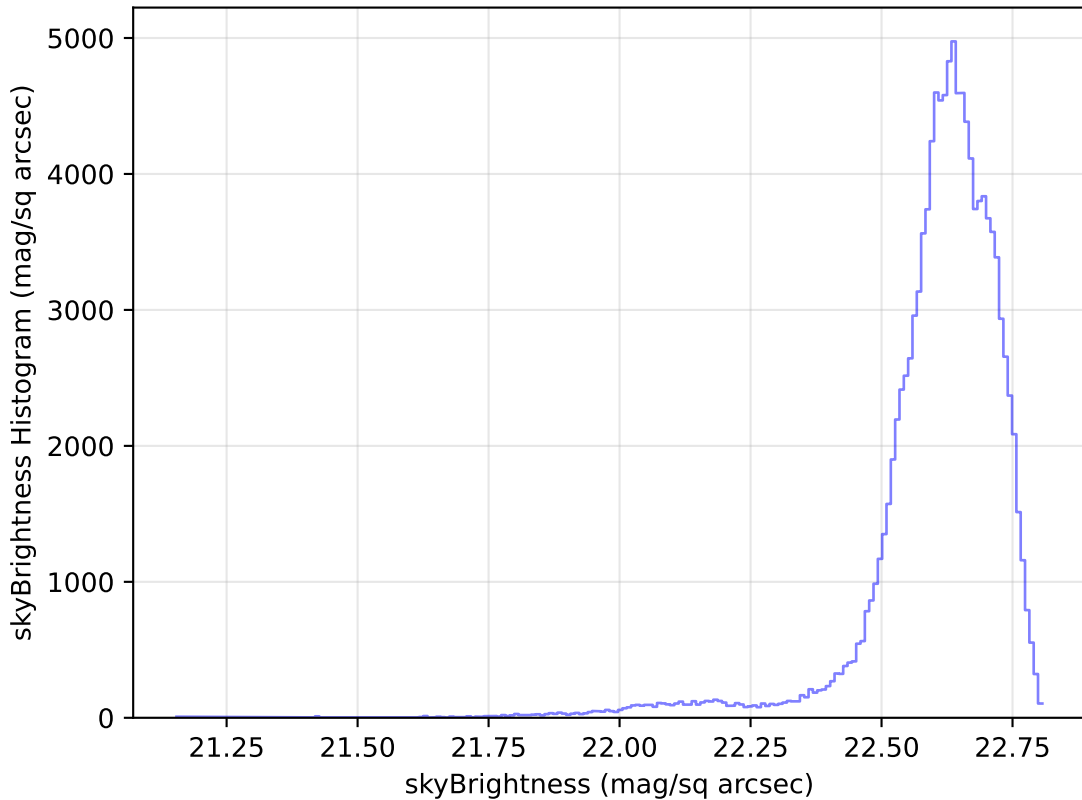
too_elab_r32_d2_gz_v3.4_10yrs All sky u band: skyBrightness Histogram
