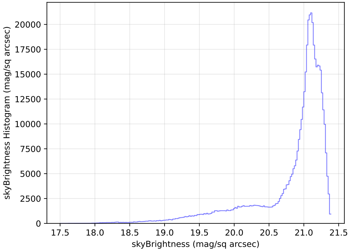
too_elab_r32_d2_gz_v3.4_10yrs All sky r band: skyBrightness Histogram
