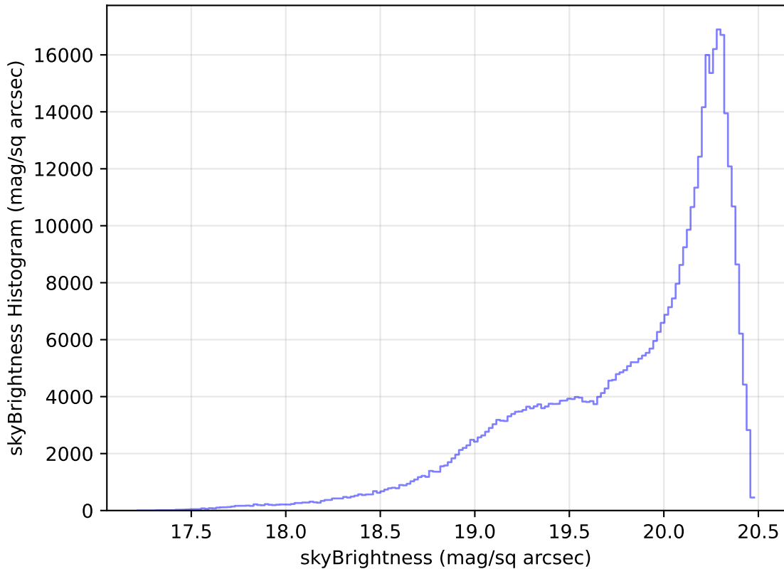
too_elab_r32_d2_gz_v3.4_10yrs All sky i band: skyBrightness Histogram
