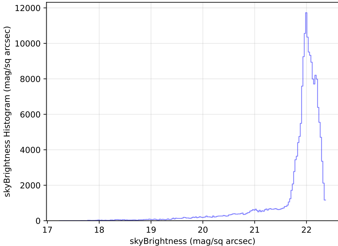
too_elab_r32_d2_gz_v3.4_10yrs All sky g band: skyBrightness Histogram
