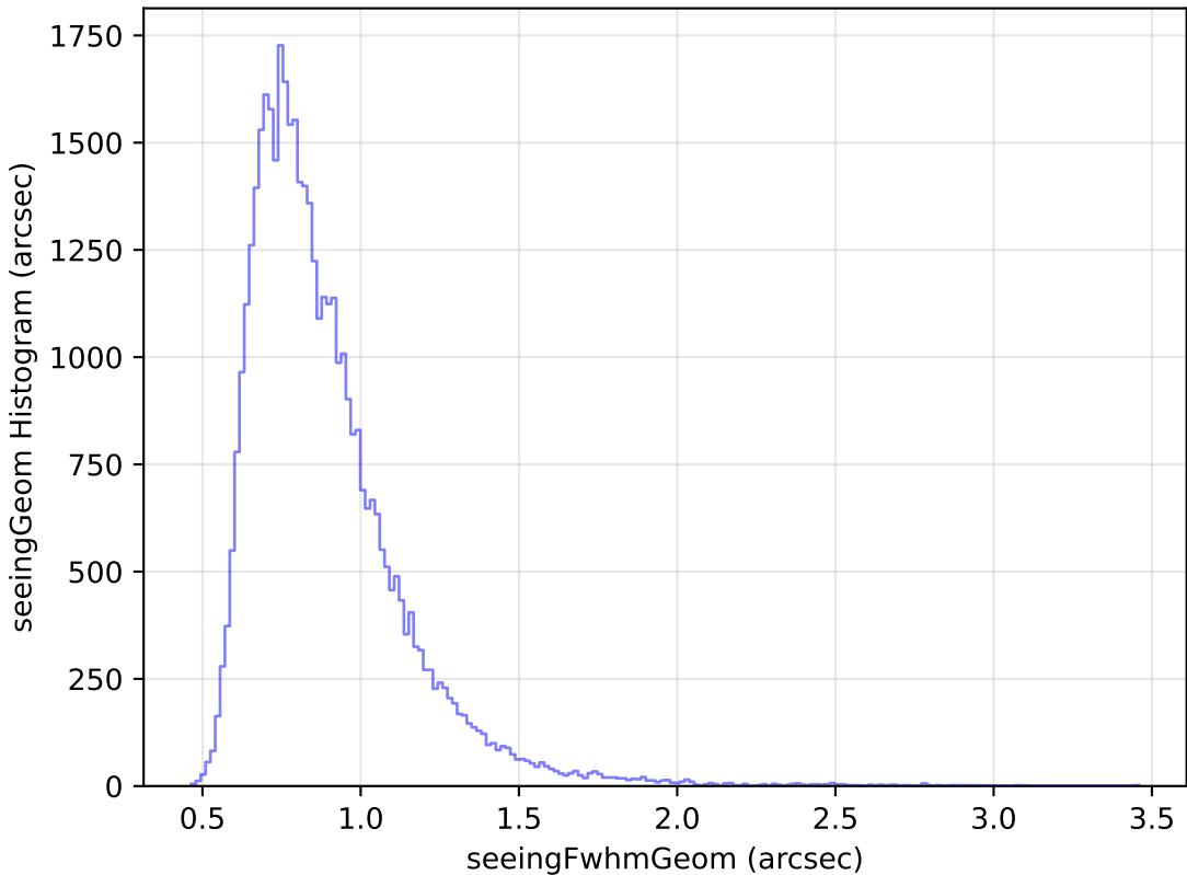
too_elab_r32_d2_gz_v3.4_10yrs Yr 1 z band: seeingGeom Histogram
