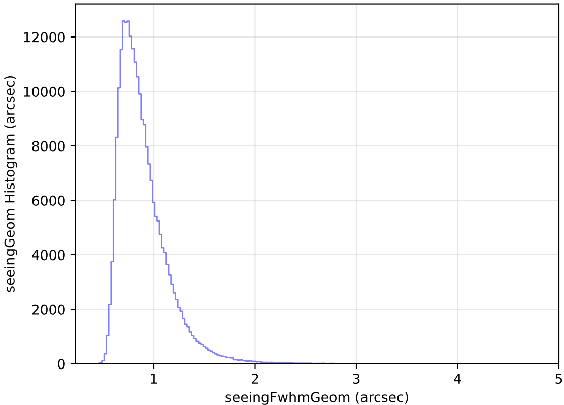
too_elab_r32_d2_gz_v3.4_10yrs Yr 1 all bands: seeingGeom Histogram
