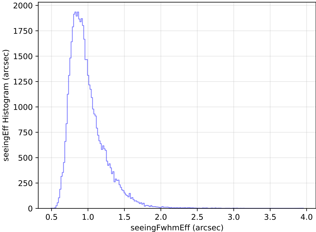
too_elab_r32_d2_gz_v3.4_10yrs Yr 1 y band: seeingEff Histogram
